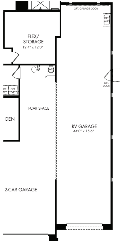
OPT. RV GARAGE EXTENSION 1 & FLEX ILO BEDROOM 4
